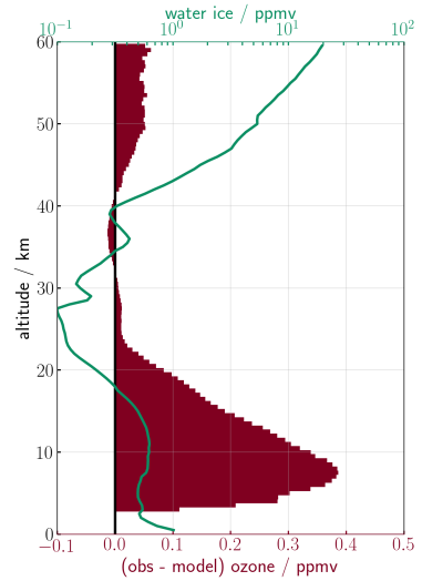
Figure 2: Averaged profiles (212 vertical profiles) > 45^\circ S between L_S = 100^\circ - 120^\circ of (green line) observed water ice, and (red bars) the difference in ozone (observed – modelled). Positive values indicate an underprediction of ozone. Modelled data are taken from the MGCM, assimilated with temperature and dust retrievals from Mars Climate Sounder.
