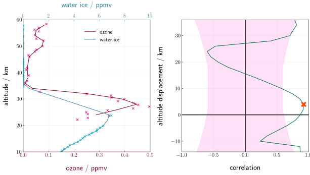
Figure 1: A cross-correlation on a pair of profiles: (left panel) vertical profiles of (blue) water ice and (red) ozone; crosses are datapoints and lines are the interpolated profiles every 2 km; (right panel) the (green) vertical correlation between the profiles across all displacements. A positive displacement of 4 km corresponds to a shifting of the water ice profile up by 4 km. The pink area marks the correlations which are not significant according to a Student’s T-test at 5% significance. The red cross indicates the most significant vertical correlation of the cross-correlation. Profiles are from NOMAD/TGO at L_S = 187^\circ , latitude 70.5^\circ S, 2020.04.21 11:04:57 UTC.
